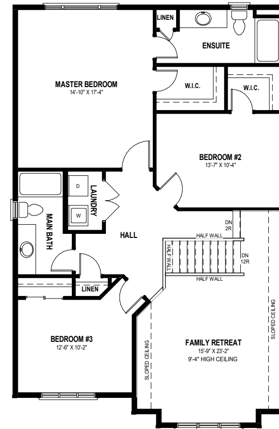
2ND FLOOR PLAN 1,347 SQ.FT
