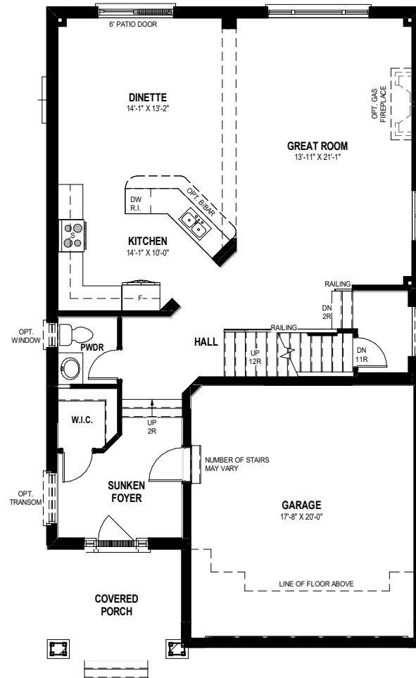
MAIN FLOOR PLAN 1,058 SQ.FT
