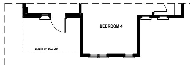
PARTIAL SECOND FLOOR PLAN ELEVATION C 1324 SQ. FT.
