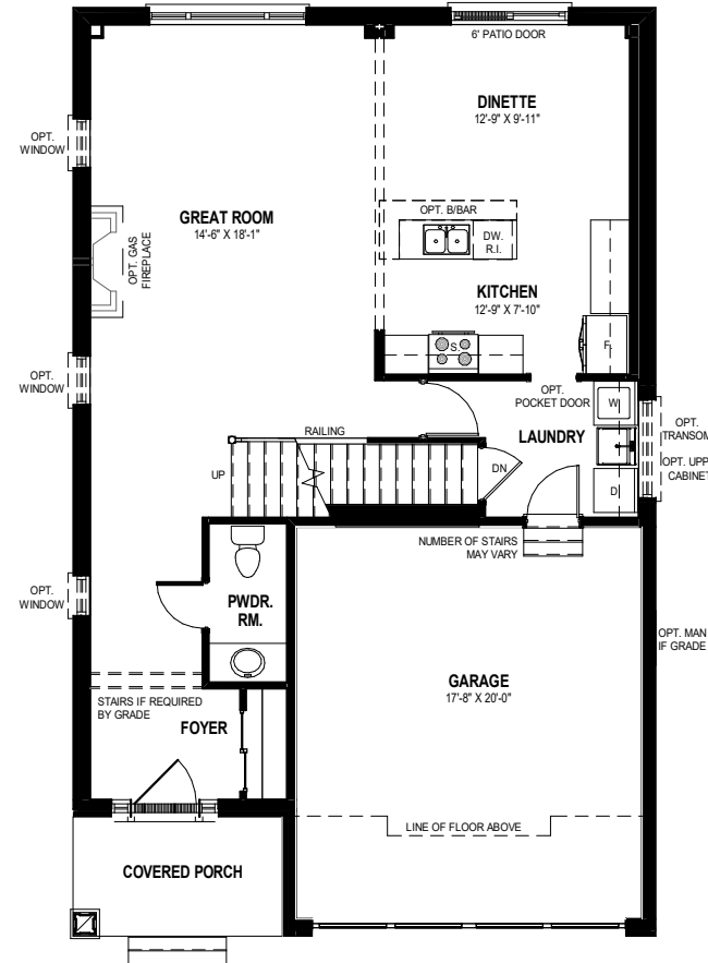
MAIN FLOOR PLAN 970 SQ. FT.
