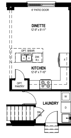
OPT. KITCHEN LAYOUT FRIDGE RELOCATED & CABINETS EXTENDED TO WALL IF PANTRY OPTION NOT SELECTED
