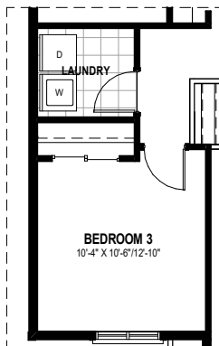
LAUNDRY C/W ALT MAIN FLOOR
