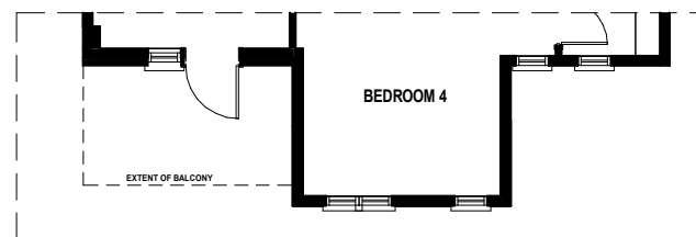
PARTIAL SECOND FLOOR PLAN ELEVATION C 1324 SQ. FT.
