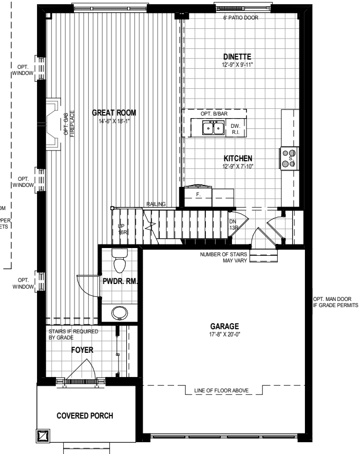
ALTERNATE MAIN FLOOR PLAN 970 SQ. FT.
