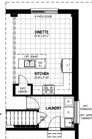
OPT. KITCHEN LAYOUT FRIDGE RELOCATED & CABINETS EXTENDED TO WALL IF PANTRY OPTION NOT SELECTED
