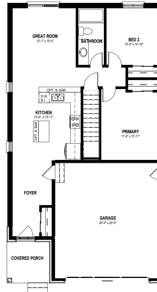
MAIN FLOOR PLAN ALT 1 1034 SQ.FT
