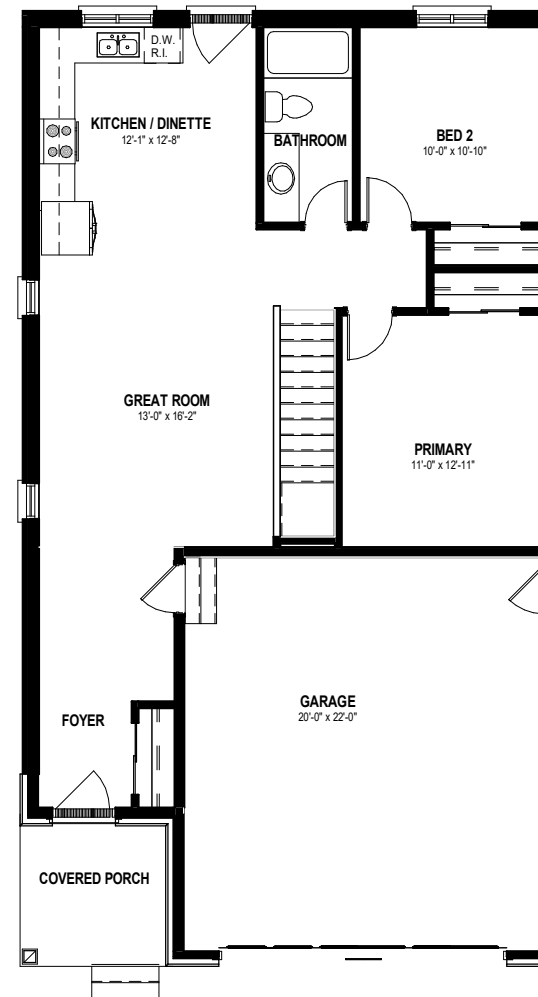
MAIN FLOOR PLAN 1034 SQ.FT
