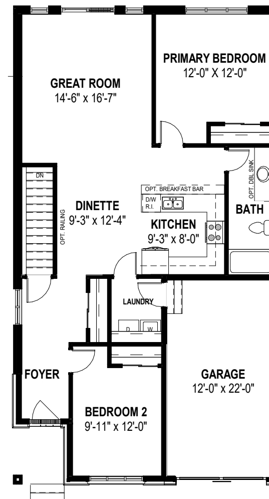
MAIN FLOOR PLAN ALT LAYOUT 1250 SQ.FT
