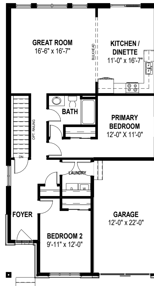
MAIN FLOOR PLAN 1250 SQ.FT
