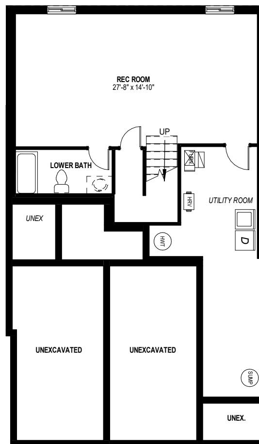
OPTIONAL FINISHED LOWER LEVEL PLAN 636 SQ. FT.
