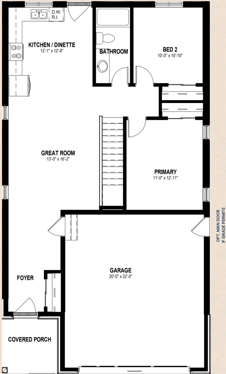
STANDARD FLOOR PLAN
