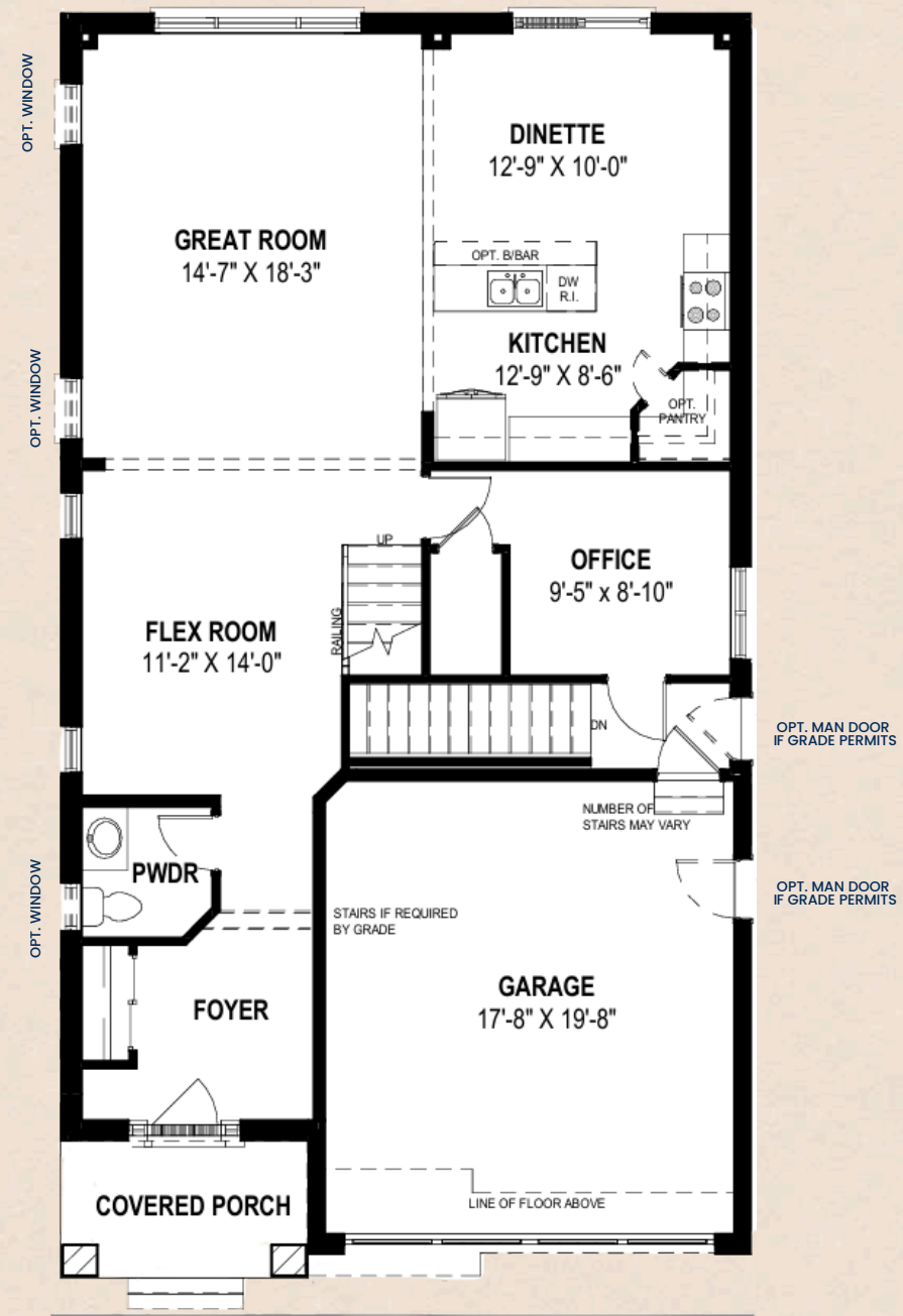
STANDARD FLOOR PLAN
