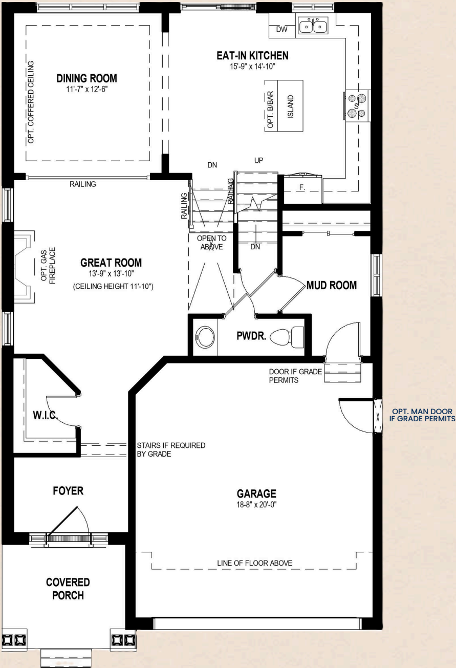
STANDARD FLOOR PLAN
